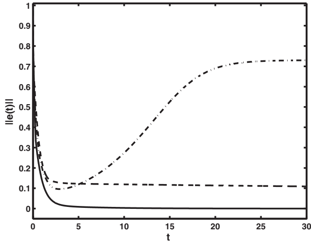
FIG. 2. Synchronization errors between network (4) and network (5) for three values of u in H with c=0.5, A=B=A_2 . The solid line corresponds to u=0.8 , the dashed line corresponds to u=1.0 , and the dash-dotted line corresponds to u=1.2 .
